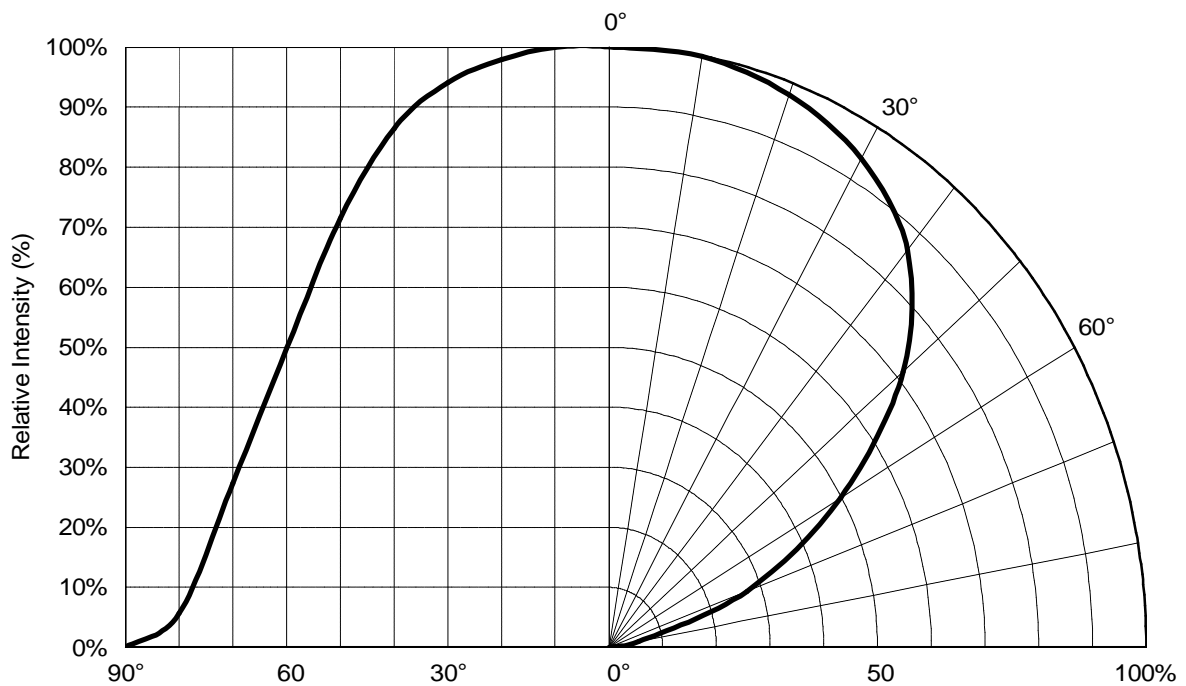
Fig 2. Radiation Characteristics
